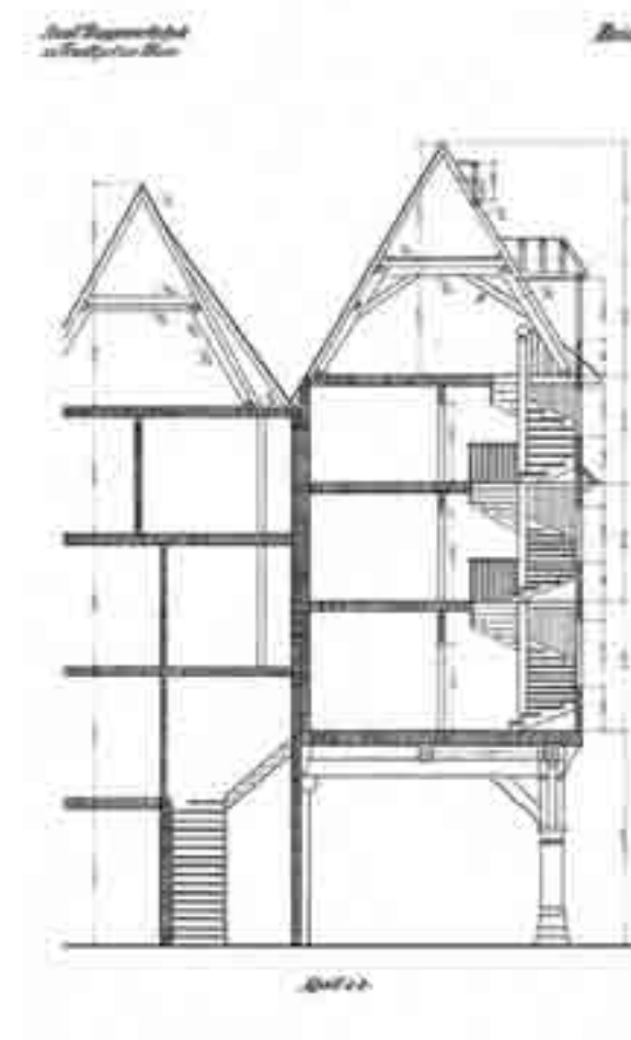
4 Schnitt Ost-West
