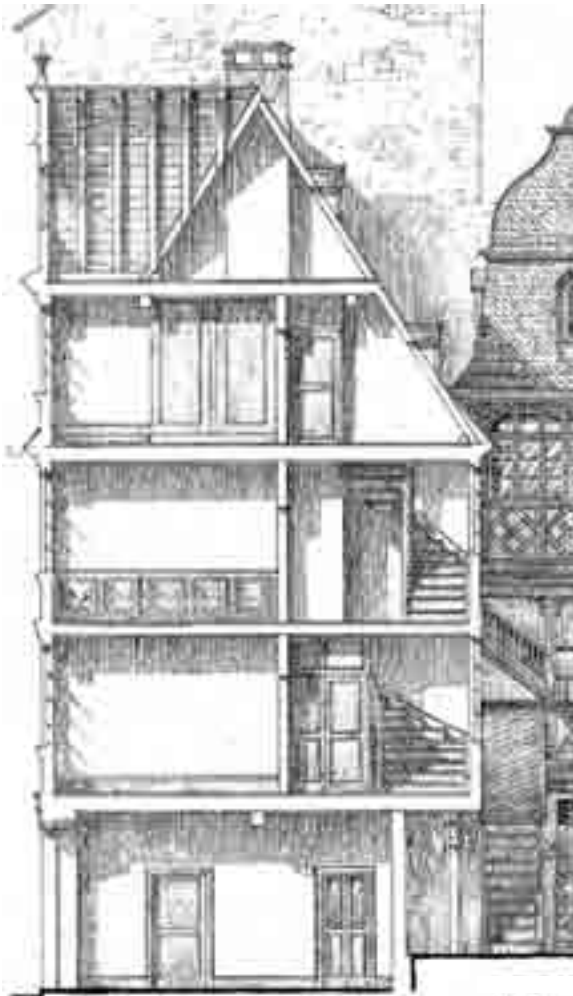
2 Schnitt Ost-West
